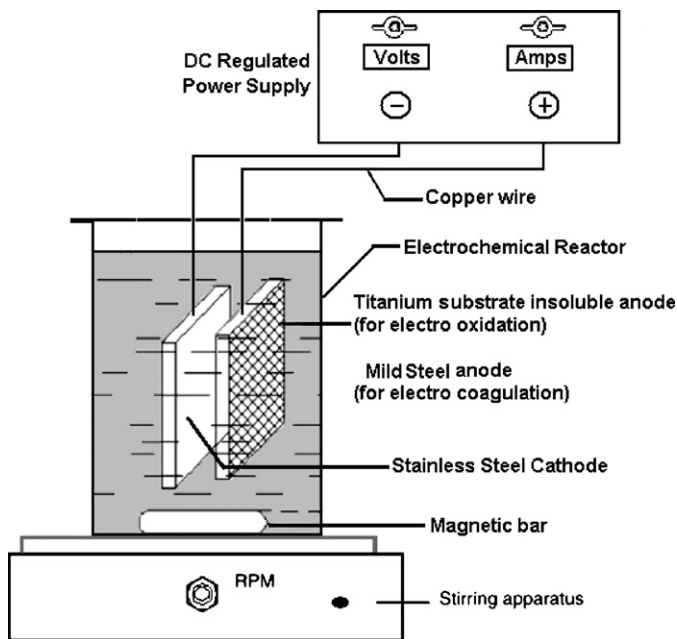
Fig. 2. Batch cell setup for electro-degradation.
